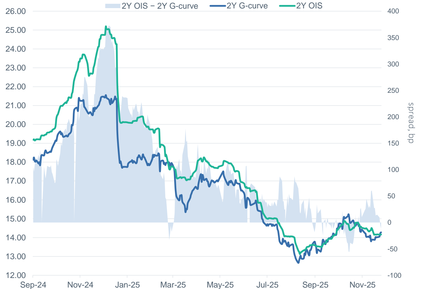
2Y G-curve and 2Y Ruonia OIS ZC in YoY basis
